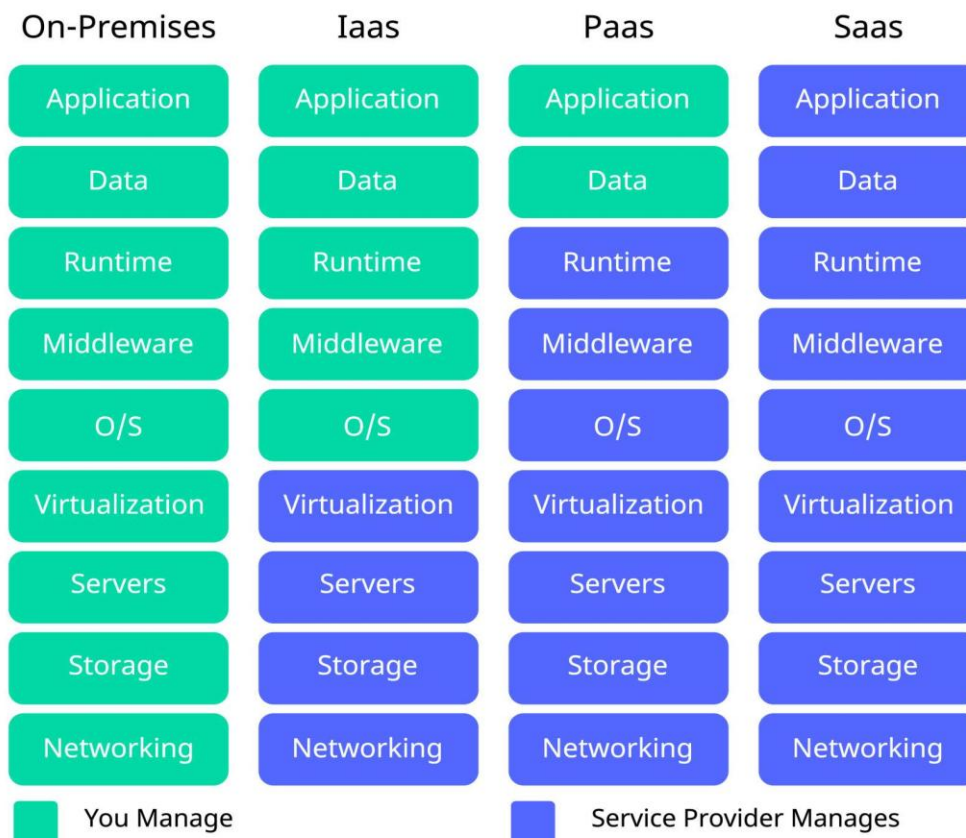
Figure 3: Cloud service models showing Infrastructure as a Service (IaaS), Platform as a Service (PaaS), and Software as a Service (SaaS).
